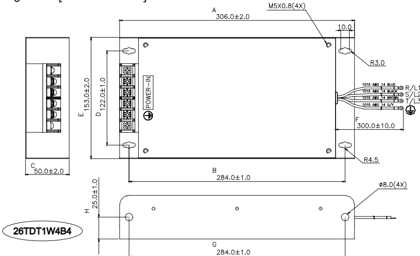
Figure 6 [ units = mm ]
