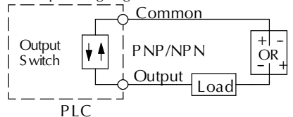
Sink/Source Output (IEC: pos./neg. logic)
