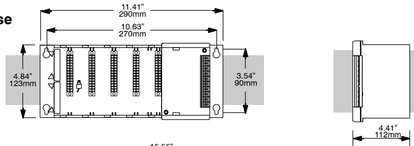
8 slot base
