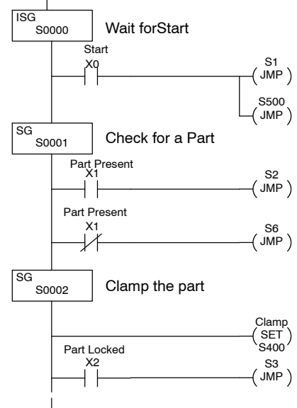
Ladder Representation
