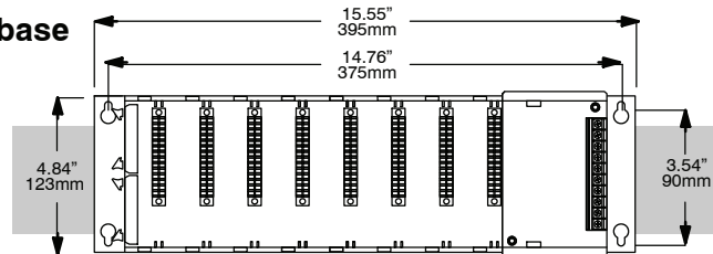
10 slot base
