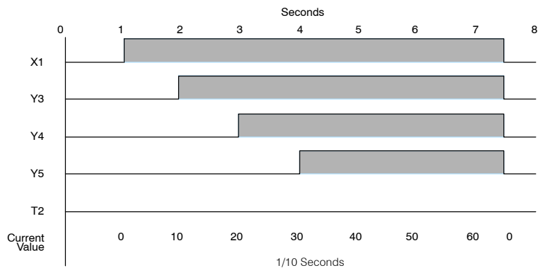
Timing Diagram
