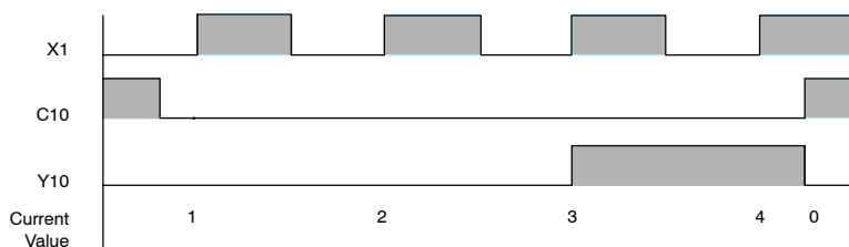
Counting diagram
