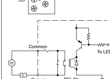
Sample Relay Output Circuit (1 of 4)
