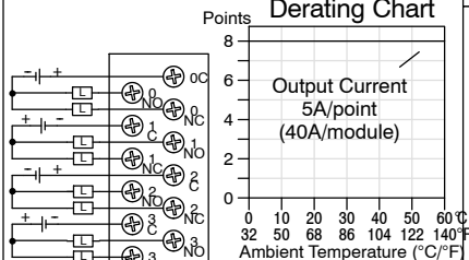
Derating Chart
