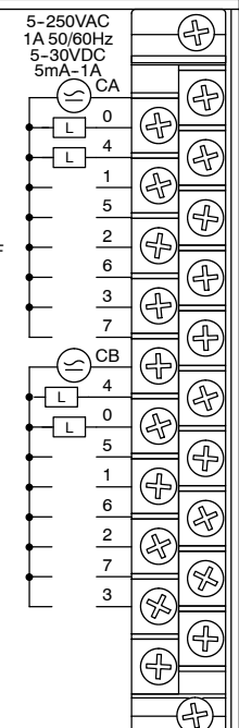
Sample Relay Output Circuit (1 of 4)
