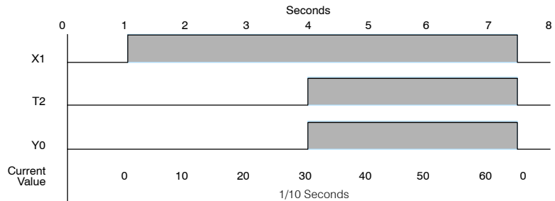
Timing Diagram
