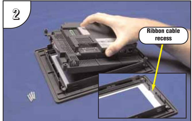
2 Lift the touch panel's main electronics housing from the front bezel. Set the front bezel and four screws to the side. Observe the ribbon cable recess on the front bezel (see detail) for use in re-assembling the panel.
