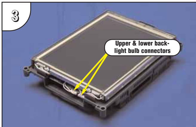
3 Place the touch panel's main electronic's housing facing up on a lint-free soft surface. Position the housing so that the backlight bulb connectors are in plain view.
