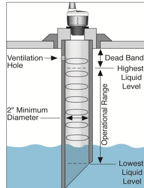
Mounting with a Standpipe
