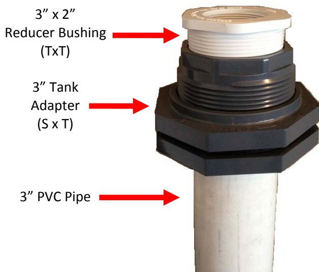
Stand-Pipe Example
