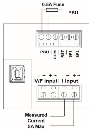
AMMETER DIRECT
