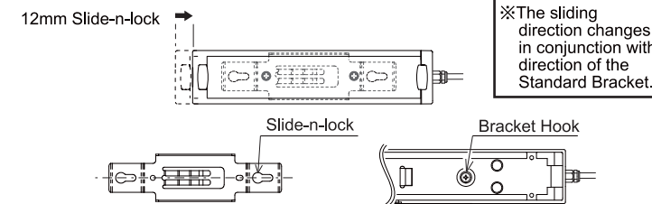
Figure 4. Slide Installation -1
