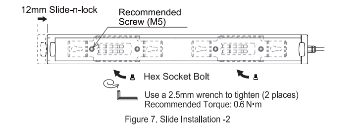
Figure 7. Slide Installation -2
