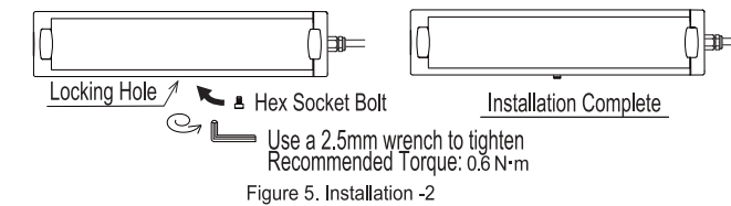
Figure 5. Installation -2
