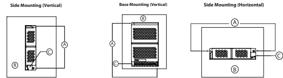
Figure 2 - Mounting
