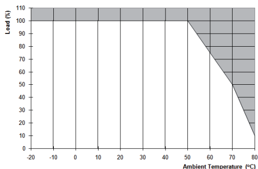
Power Derating Curve for PSU
