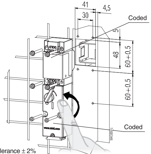
Dimension tolerance \pm 2\%
