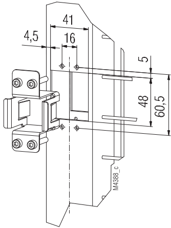
Dimension tolerance \pm 1\% Frame profile 50 mm x 50 mm
