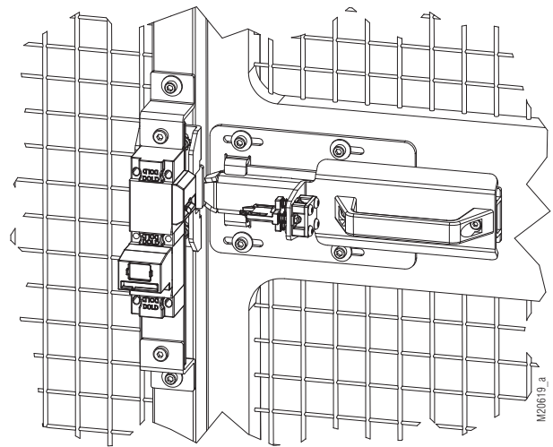
Installation dimensions see 2.7 Actuator module B + actuator CW
