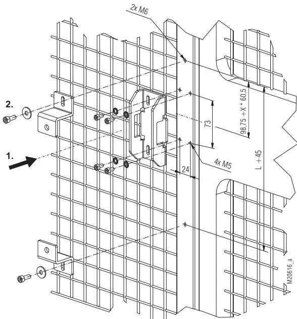
Installation dimensions see 2.7 Actuator module B + actuator CW
