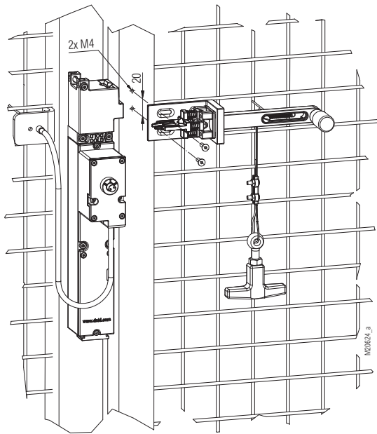
Installation dimensions see 2.7 Actuator module B + actuator CS
