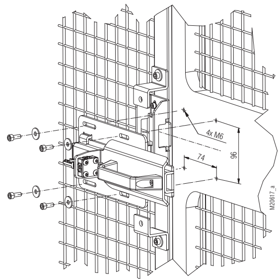
Installation dimensions see 2.7 Actuator module B + actuator CW
