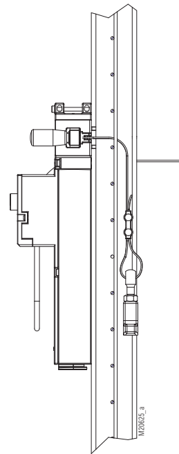
Lead wire rope and T-handle through the grid
