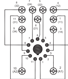
WIRING DIAGRAM TOP VIEW
