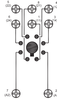
WIRING DIAGRAM TOP VIEW
