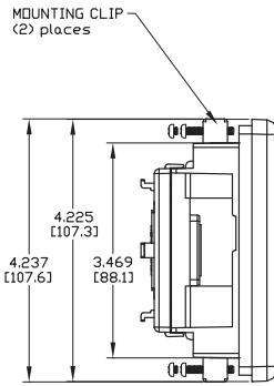
LEFT VIEW
