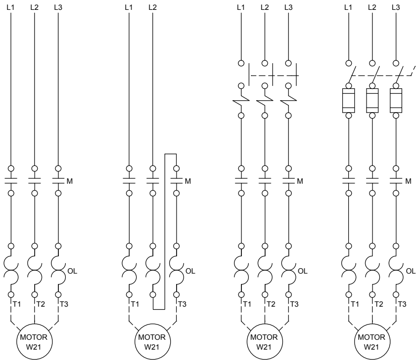
NON COMBINATION 3-PHASE
