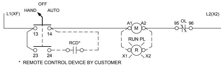
HAND - OFF - AUTO SELECTOR SWITCH
