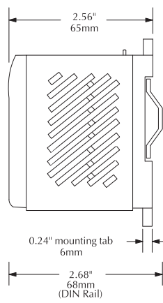
Mounting orientation
