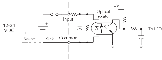
Equivalent input circuit, high-speed inputs (X0-X2)
