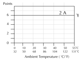
Derating chart for relay outputs
