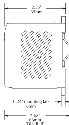
Mounting orientation
