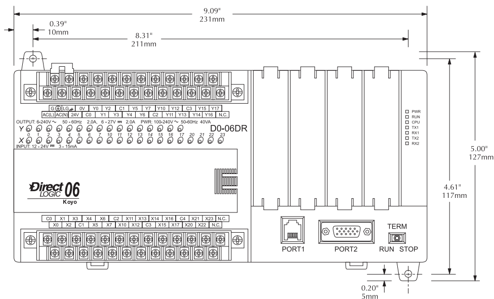
Mounting orientation
