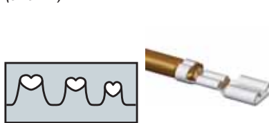
Fig. 5 (BM-531) Barrel Open Terminals 20-10 AWG (0.5-6 mm 2 )
