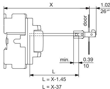
PISTOL HANDLE TYPE G FBCC30CDT - FBJ30CDT
