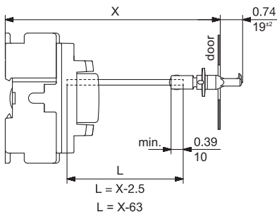
PISTOL HANDLE TYPE D FBCC30CDT - FBJ30CDT
