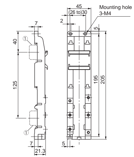
①35mm wide rail (height 15mm) x 2
