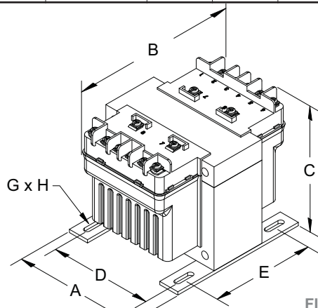
FIGURE B (150VA to 1500VA)
