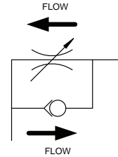
Inch/Metric Flow Control Valve
